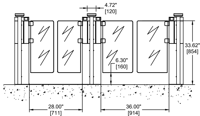
ELEVATION VIEW
