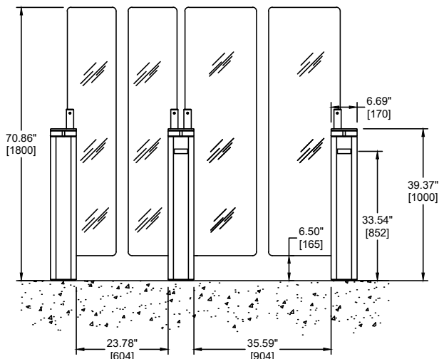
ELEVATION VIEW
